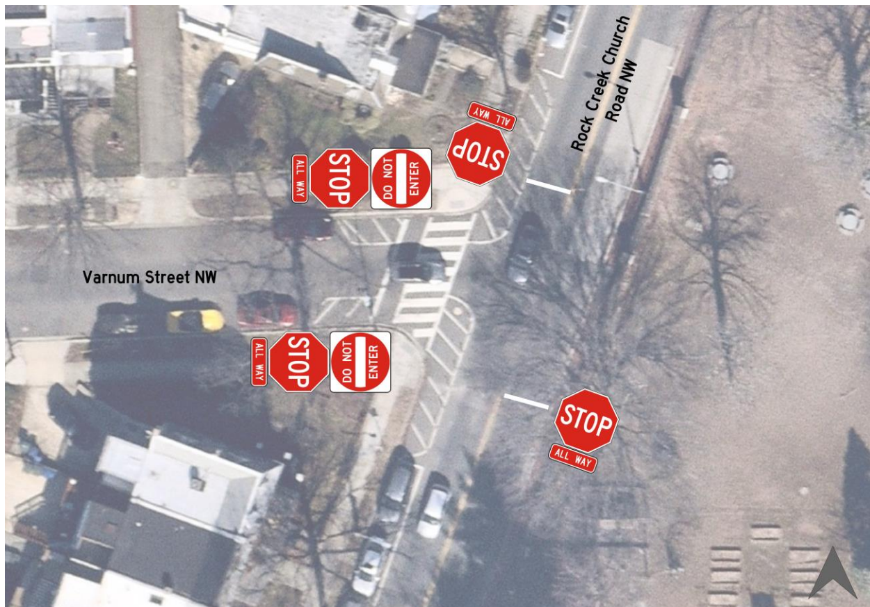
Figure 1: Proposed Signs and Markings at Rock Creek Church Road and Varnum Street NW
