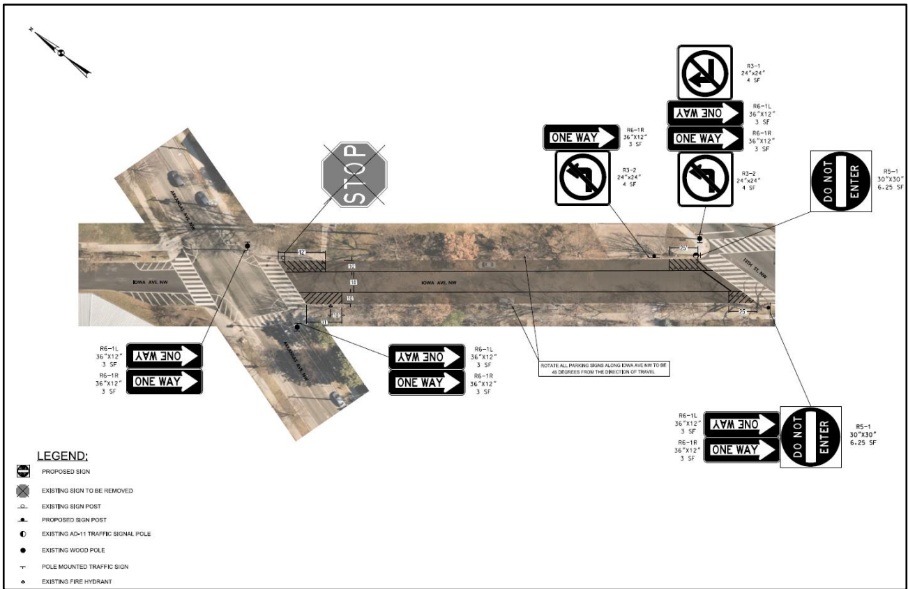
Figure 1: Conceptual Improvements for Conversion of Iowa Avenue to One-Way Southeast-bound from Arkansas Avenue to 13th Street NW
