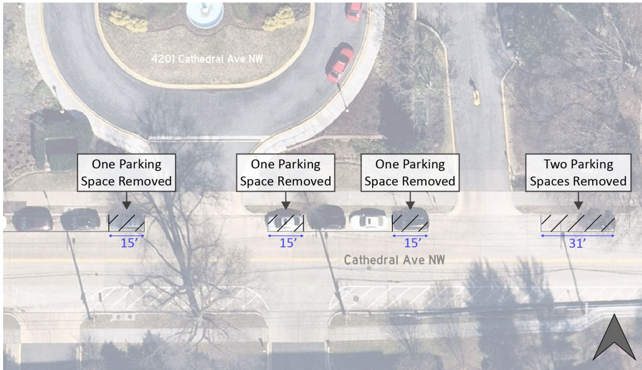
Figure 1 | Proposed Parking Removal and Pavement Marking for Cathedral Avenue NW
