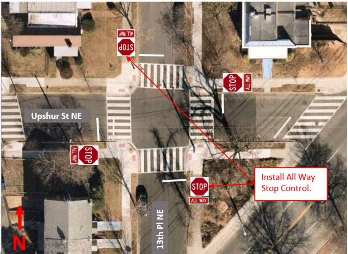
Figure 1: Proposed Improvements at 13 th Place NE and Upshur Street NE
