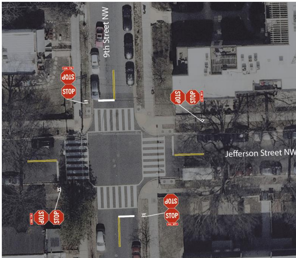
Figure 1: Proposed Improvements at 9 th Street and Jefferson Street NW
