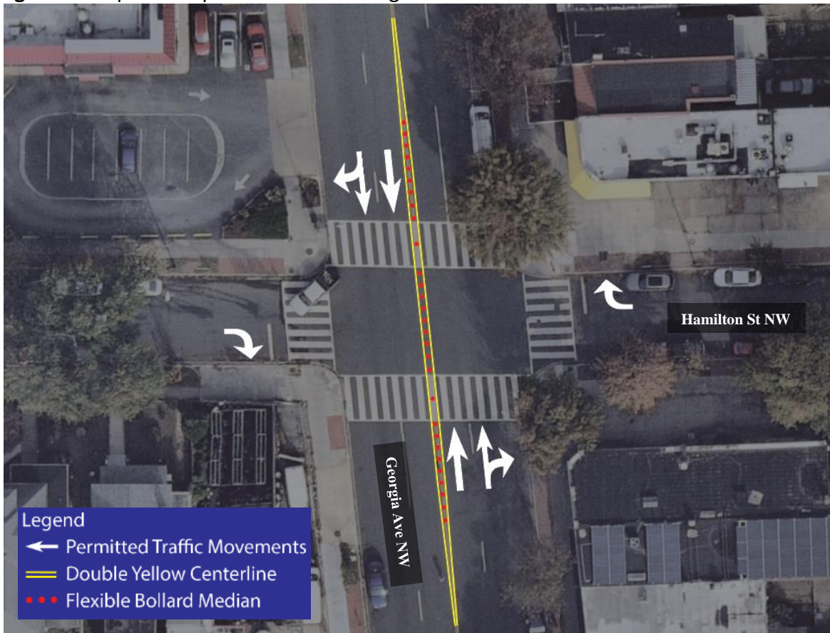
Figure 1: Proposed Improvements at Georgia Avenue and Hamilton Street NW Intersection
