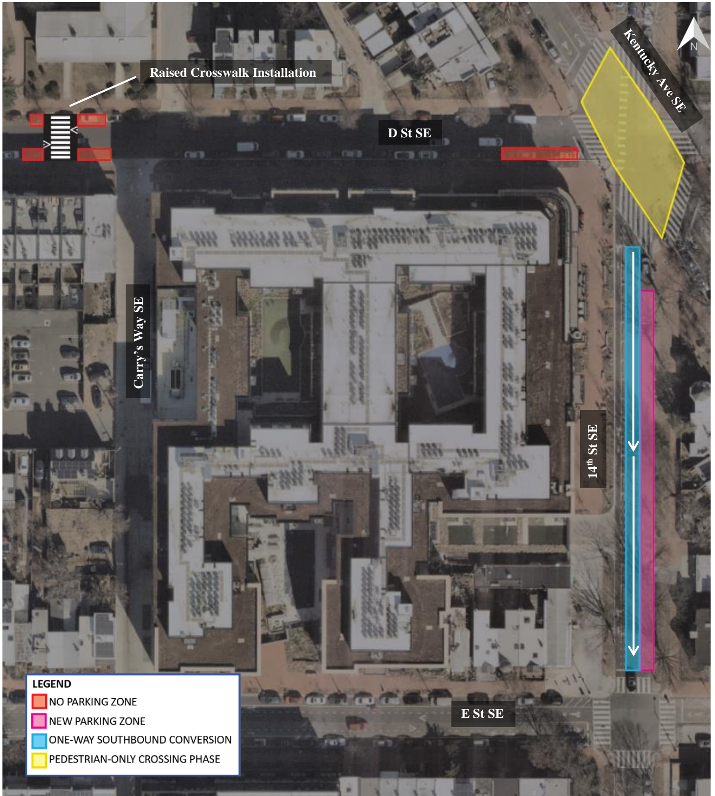
Figure 1: Full Extent of Proposed Improvements at Intersection
