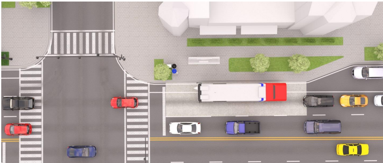
Figure 34-1 | Near-Side Bus Stop Location
