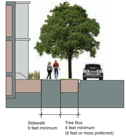
Typical Residential Cross-Section (Low and Moderate Density Residential)
