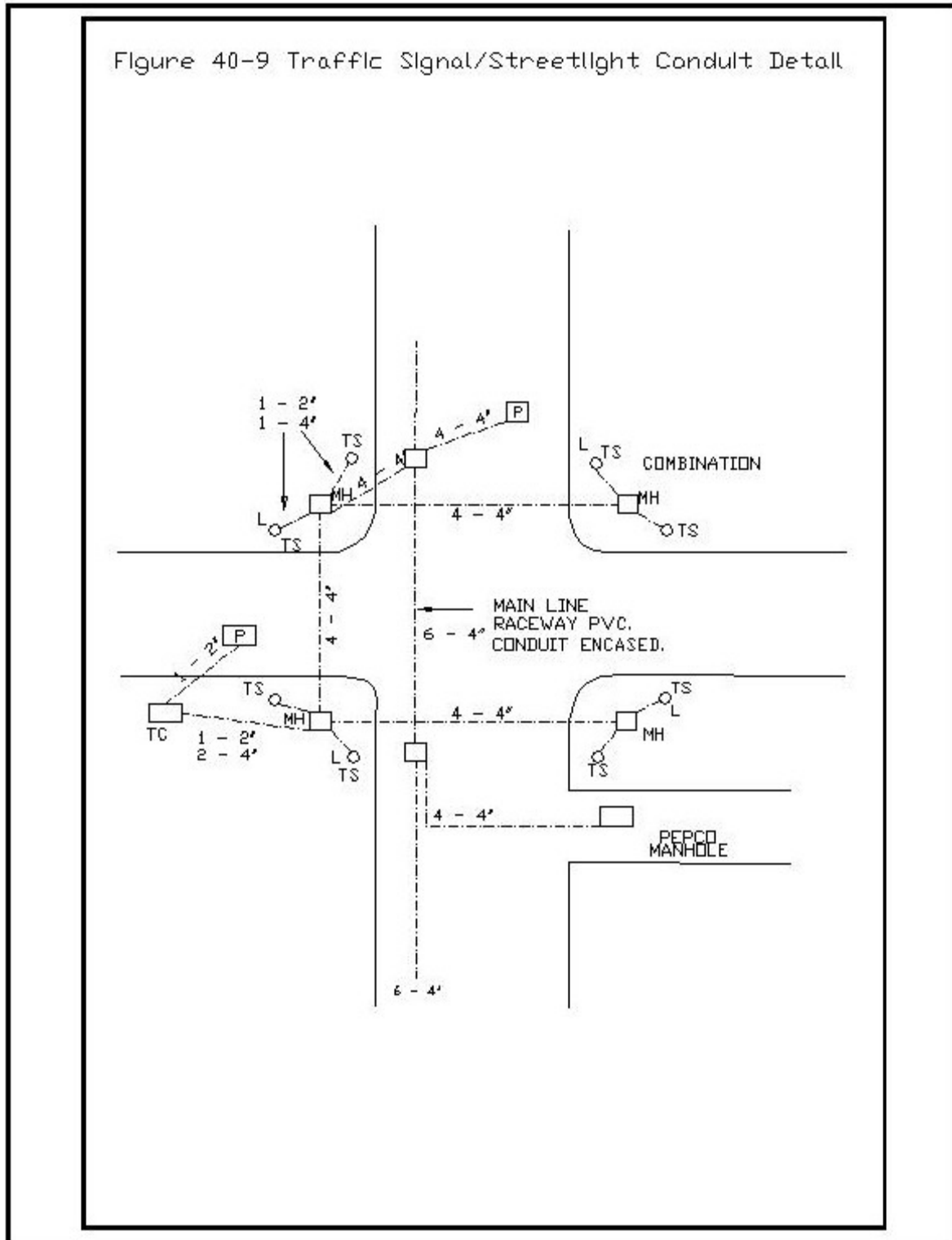
Figure 40-9. Traffic Signal and Streetlight Conduit Detail
