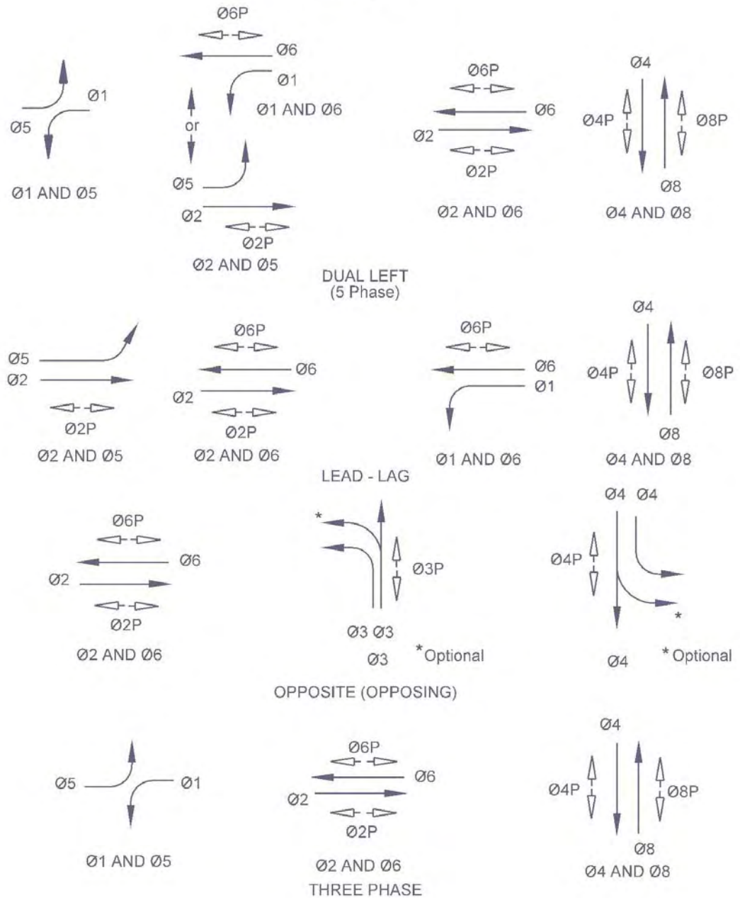
Figure 40-7 LEFT-TURN PHASING METHODS (Phase Diagrams)
