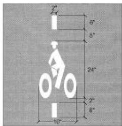
BICYCLE DETECTION SYMBOL
