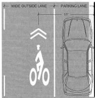
WIDE OUTSIDE LANE ADJACENT TO PARKING
