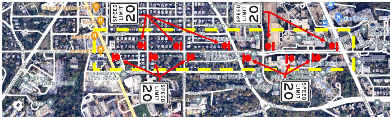
Figure 1: proposed improvements on Van Ness Street, NW, between Connecticut Avenue and Wisconsin Avenue
