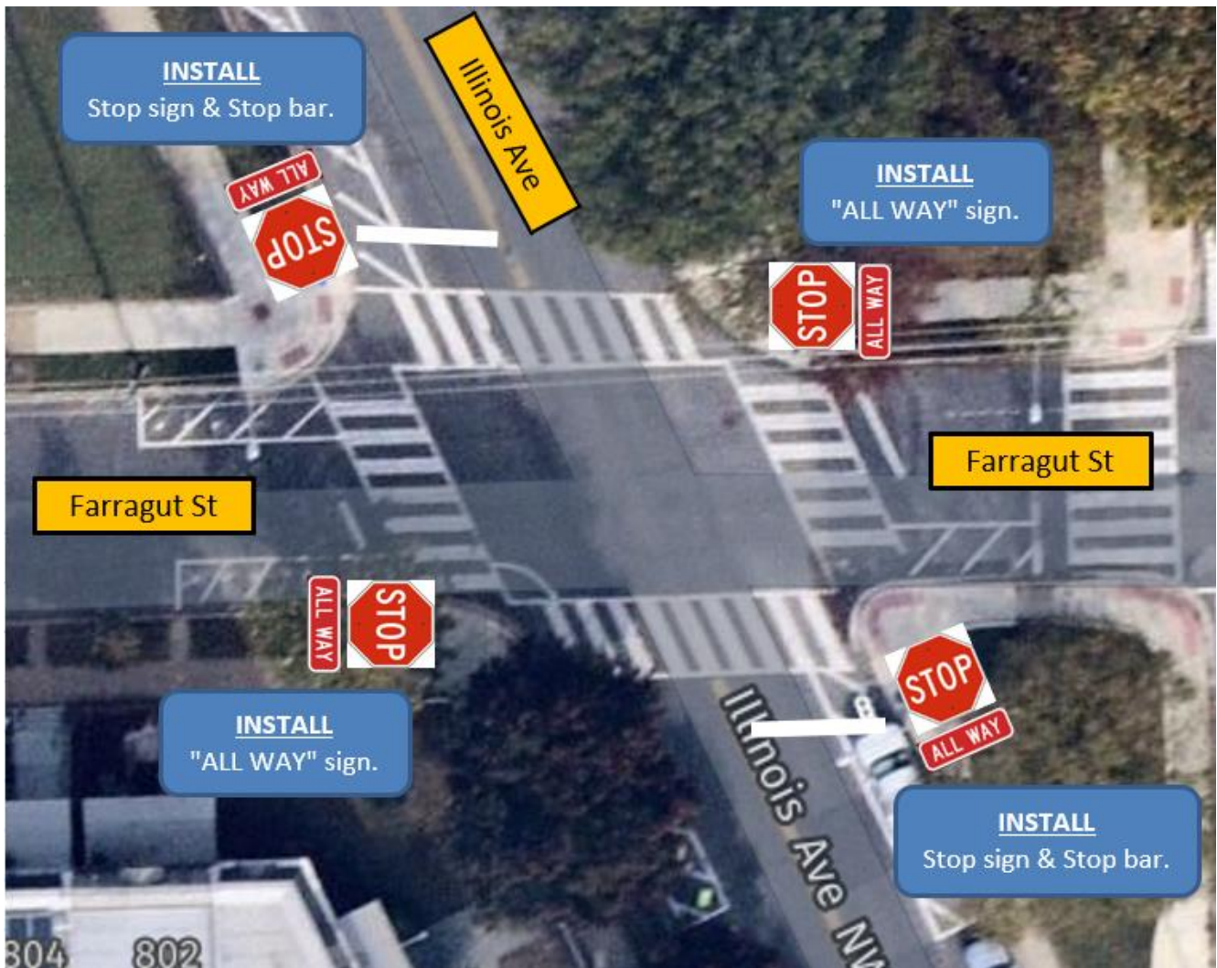
Figure 1: Proposed Improvements at Illinois Ave & Farragut St NW
