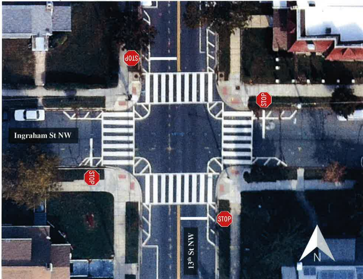
Figure 1: Proposed Improvements at 13 th and Ingraham Streets NW
